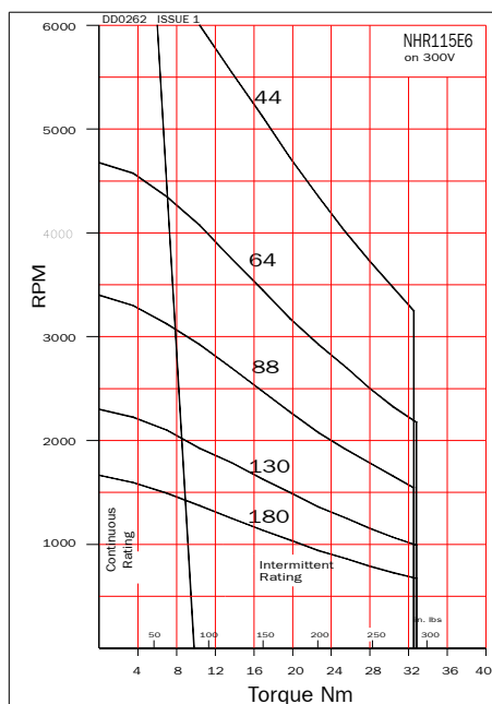
NHR115E6 on 300V
