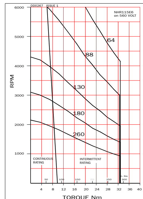
NHR115E6 on 560V
