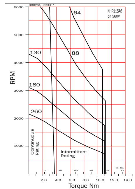
NHR115A6 on 560V
