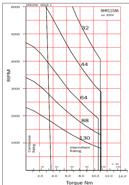
NHR115A6 on 300V
