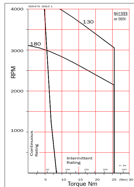
NHJ130E8 on 560V
