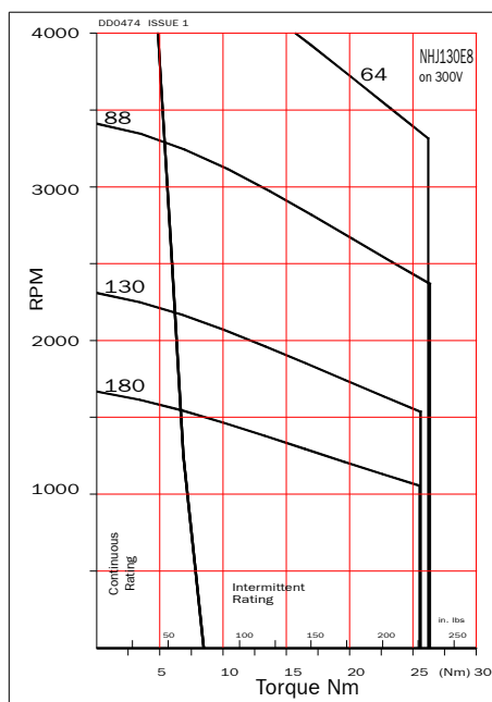
NHJ130E8 on 300V
